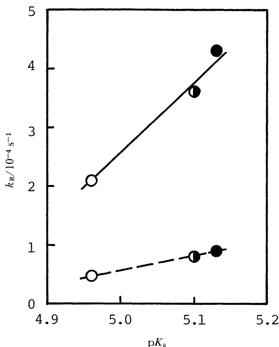
Fig. 1. Rate constant for racemization in carboxylic acids. pK a : The value at 100 °C was estimated from data 0–60 °C. —: (R)-2-Phenylglycine (1.00 mmol). ---: (R)-2-(4-Hydroxyphenyl)glycine (1.00 mmol). (1RS,4SR)-10-Camphorsulfonic acid: 0.95 mmol. Temperature: 100 °C. Solvent: Mixture of 30 cm 3 of carboxylic acid and 3 cm 3 of water. k R : Rate constant for racemization. Carboxylic acid: ○ Acetic acid; ● propanoic acid; ● butanoic acid.
