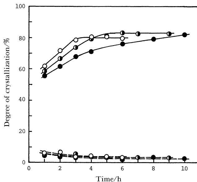
Fig. 2. Influence of amount of (1S)-10-camphorsulfonic acid on asymmetric transformation. (RS)-2-Phenylglycine [(RS)-Phg]: 20.0 mmol. (1S)-10-Camphorsulfonic acid [(S)-CS]: ○ 18.0 mmol; ● 19.0 mmol; ● 20.0 mmol. Solvent: 10 cm 3 of butanoic acid. Temperature: 100 °C. —: Salt of (R)-Phg with (S)-CS. ---: Salt of (S)-Phg with (S)-CS.
